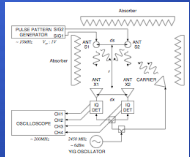
Experimental setup for blind source separation
