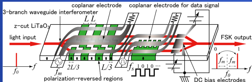
Basic structure of FSK modulator using 3-branch WG interferometer & pol.-rev. structure
